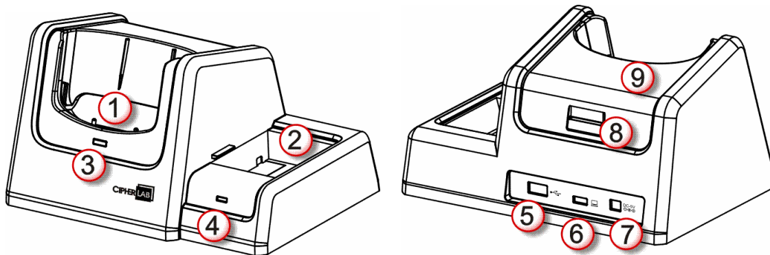
Figure 14: Cradle Overview
